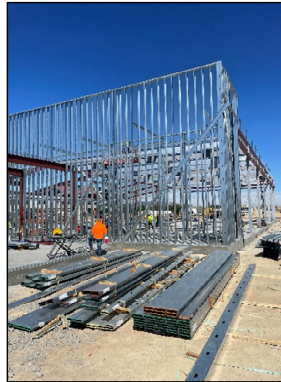
Steel Frame
