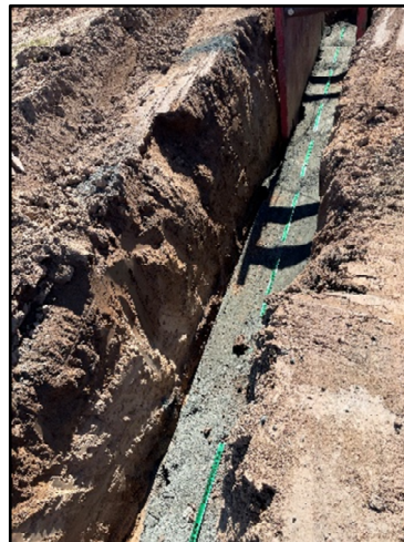
Sewer Backfill
