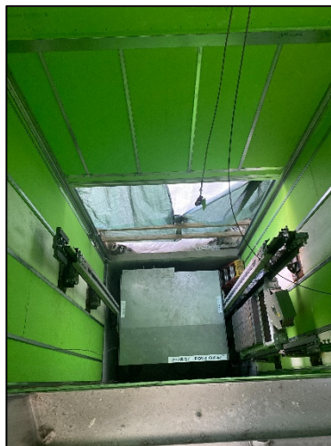
Elevator Installation
