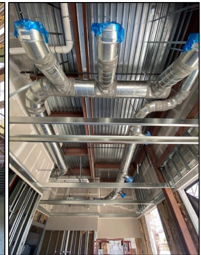
HVAC Rough In 2 nd Floor
