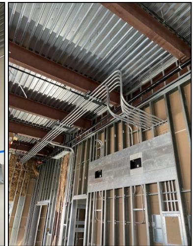
Electrical Rough In 2 nd Floor
