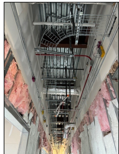
Cable Tray – 1 st Floor
