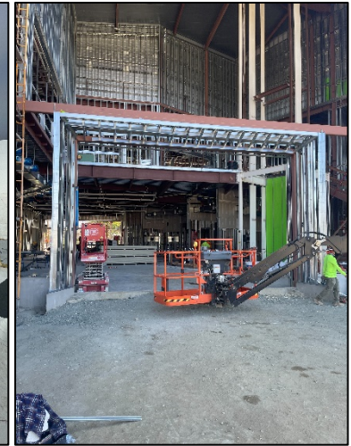
Entrance Wing Wall Framing
