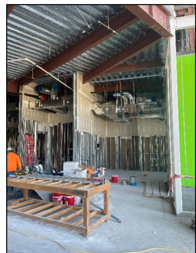
1 st Floor HVAC Ducting
