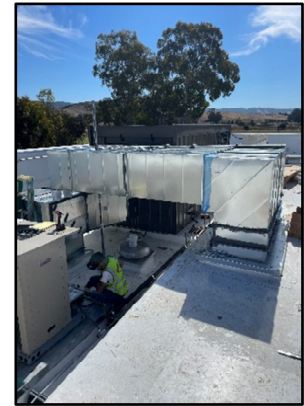
MZU Supply Ducting
