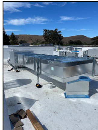
MAF-1 Duct
