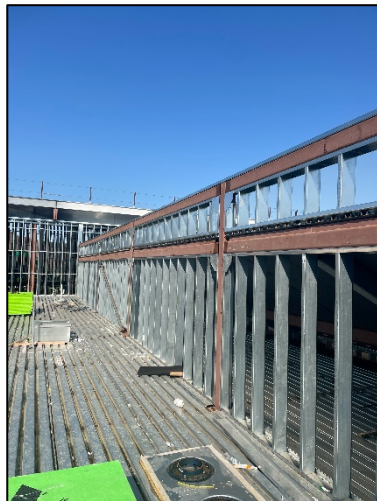
Roof Parapet Wall Framing
