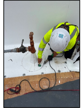
Welding Single Ply
