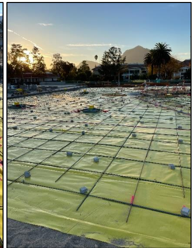
Under Slab Vapor Barrier & Rebar (West Side)
