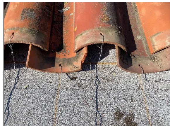
Wire Tie System
