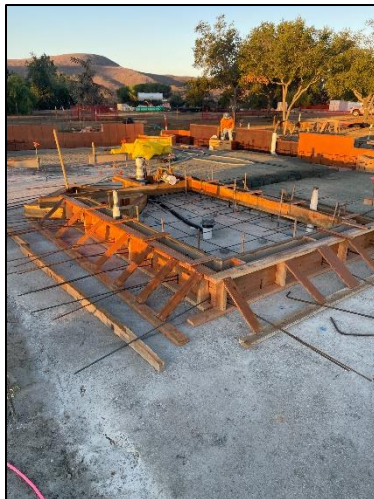
Restroom Wall Curb (West)
