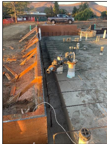
Perimter Wall Footing Form Boards (West Side)
