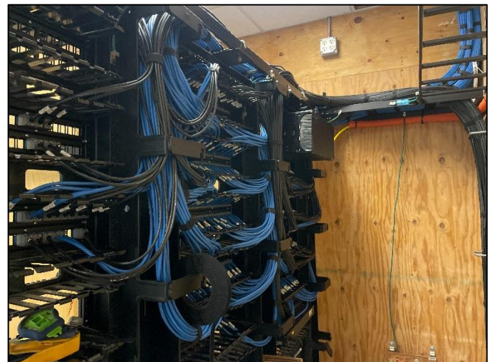
IDF Terminations
