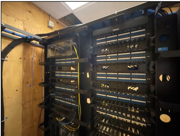
IDF Rack
